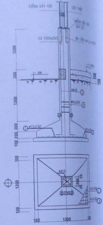
MÓNG M2 (4CK)
